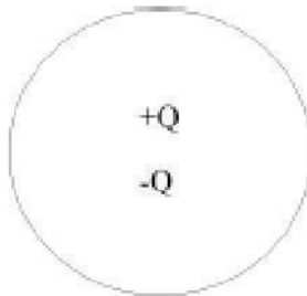
Fig: Atom of an Dielectric
